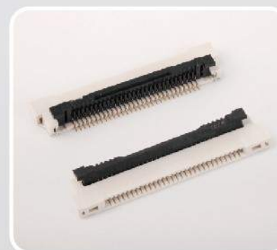
0.5mm (.020") SMT TYPE
