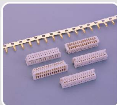
1.25mm (.049") ■ Housing : JS-2255(Double row) Terminal : JS-2255-T / TG ■ Poles : 20,30,40
