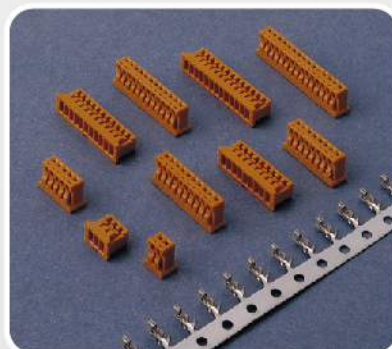
1.25mm (.049") ■ Housing : JS-1250 Wafer : JS-1251(180°) JS-1251R(90°) Terminal : JS-1250-T ■ Poles : 02-15
