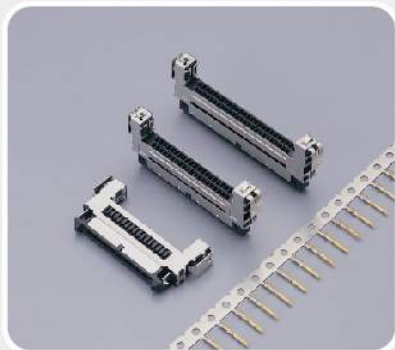
1.0mm(.039") ■ Housing : JS-2015 Terminal : JS-2015-TG ■ Poles : 31
